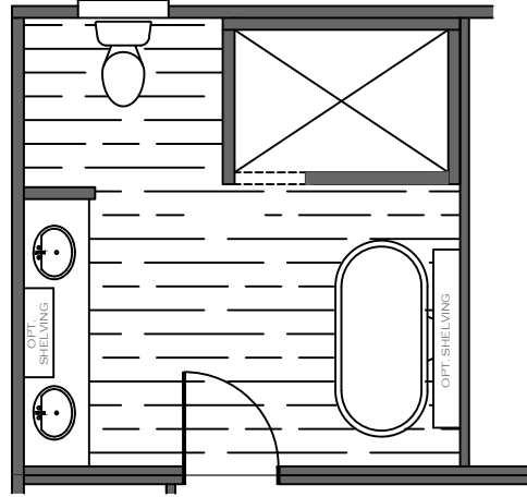
OPT. PRIMARY BATH W/ 72" SHOWER
