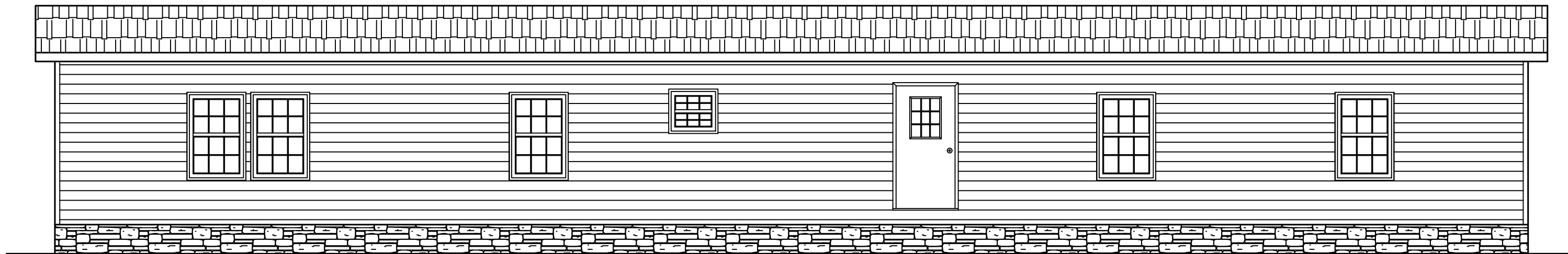
76'-0" REAR ELEVATION
