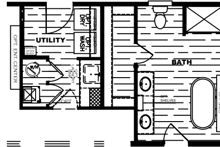
OPT. DOUBLE PRIMARY BATHROOM & UTILITY ROOM
